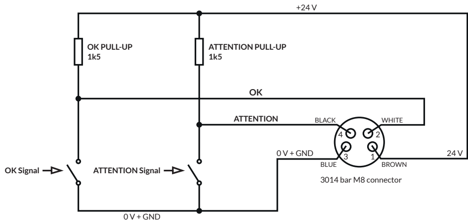
Circuit inside the 3014
