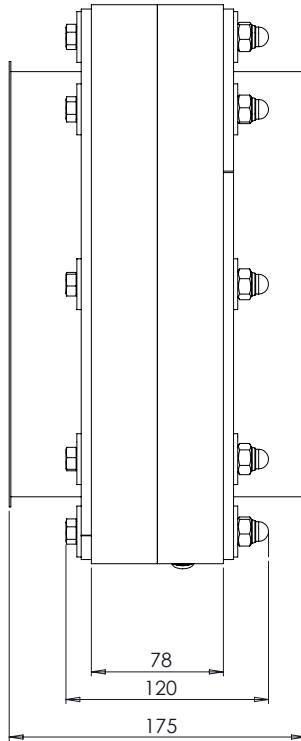
302414-250 Side View
