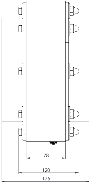
302414-200 Side View
